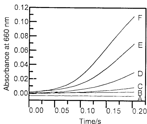
Fig. 6 Kinetic traces showing the induction period for the formation of \text{ABTS}^{+\cdot} monitored as a function of time at 660 nm at varying hydrogen peroxide concentrations in 0.05 M phosphate buffer at pH 7.0: [\text{L}^{\text{I}}\text{Fe}^{\text{II}}] = 2.8 \times 10^{-4} , [\text{ABTS}] = 1.0 \times 10^{-3} , [\text{H}_2\text{O}_2] = 0 (trace A), 3.85 \times 10^{-4} (B), 7.65 \times 10^{-4} (C), 11.5 \times 10^{-4} (D), 15.3 \times 10^{-4} (E) and 19.1 \times 10^{-4} \text{ M} (F). Experimental conditions: ionic strength = 0.20 M (phosphate buffer); T = 25.0 \pm 0.2^\circ\text{C} .
