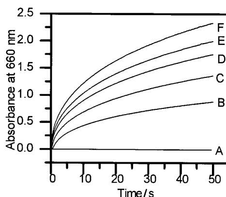
Fig. 5 Reaction traces for the formation of \text{ABTS}^{+\cdot} recorded at 660 nm at different concentrations of hydrogen peroxide. Experimental conditions: [phosphate buffer] = 0.05 M; pH 7.0; [\text{L}^1\text{Fe}^{\text{II}}] = 2.8 \times 10^{-4} M, [\text{ABTS}] = 1.0 \times 10^{-3} M, [\text{H}_2\text{O}_2] = 0 (trace A), 3.85 \times 10^{-4} (B), 7.65 \times 10^{-4} (C), 11.5 \times 10^{-4} (D), 15.3 \times 10^{-4} (E) and 19.1 \times 10^{-4} M (F); ionic strength = 0.20 M (phosphate buffer); T = 25.0 \pm 0.2^\circ\text{C} .
