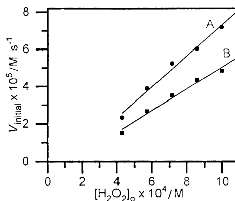
Fig. 8 Dependence of initial rates of formation of \text{ABTS}^{+\cdot} ( V_{\text{initial}}/\text{M s}^{-1} ) on the initial concentration of hydrogen peroxide. Plot A was obtained in the presence of 36 \mu\text{M} [\text{L}^{\text{I}}\text{Fe}^{\text{II}}] , B in the presence of 91 \mu\text{M} [\text{L}^{\text{II}}\text{Fe}^{\text{II}}] . Experimental conditions: [\text{ABTS}] = 0.01 \text{ M} ; [phosphate] = 0.05 M (pH 7); T = 25.0 \pm 0.2^\circ\text{C} ; ionic strength = 0.20 M (phosphate buffer).
