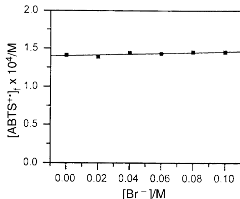
Fig. 7 Dependence of [\text{ABTS}^{+\cdot}]_f on the bromide ion added during the scavenging of \text{L}^{\text{I}}\text{Fe}^{\text{IV}}=\text{O} by ABTS in 0.05 M phosphate buffer at pH 7.0. [\text{L}^{\text{I}}\text{Fe}^{\text{II}}] = 2.8 \times 10^{-4} \text{ M} , [\text{ABTS}] = 1.0 \times 10^{-3} \text{ M} , [\text{H}_2\text{O}_2] = 1.53 \times 10^{-3} \text{ M} , ionic strength = 0.30 M (phosphate buffer and NaCl or NaBr); T = 25.0 \pm 0.2^\circ\text{C} .
